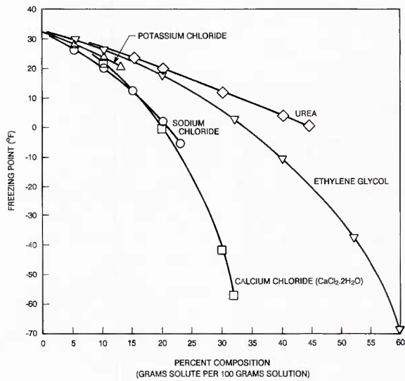
Figure 3-1 Freezing point of aqueous solutions.
